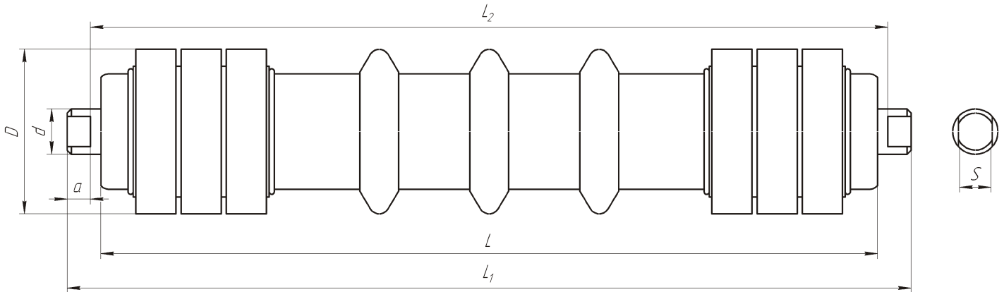
Figure 1 Disk roller
