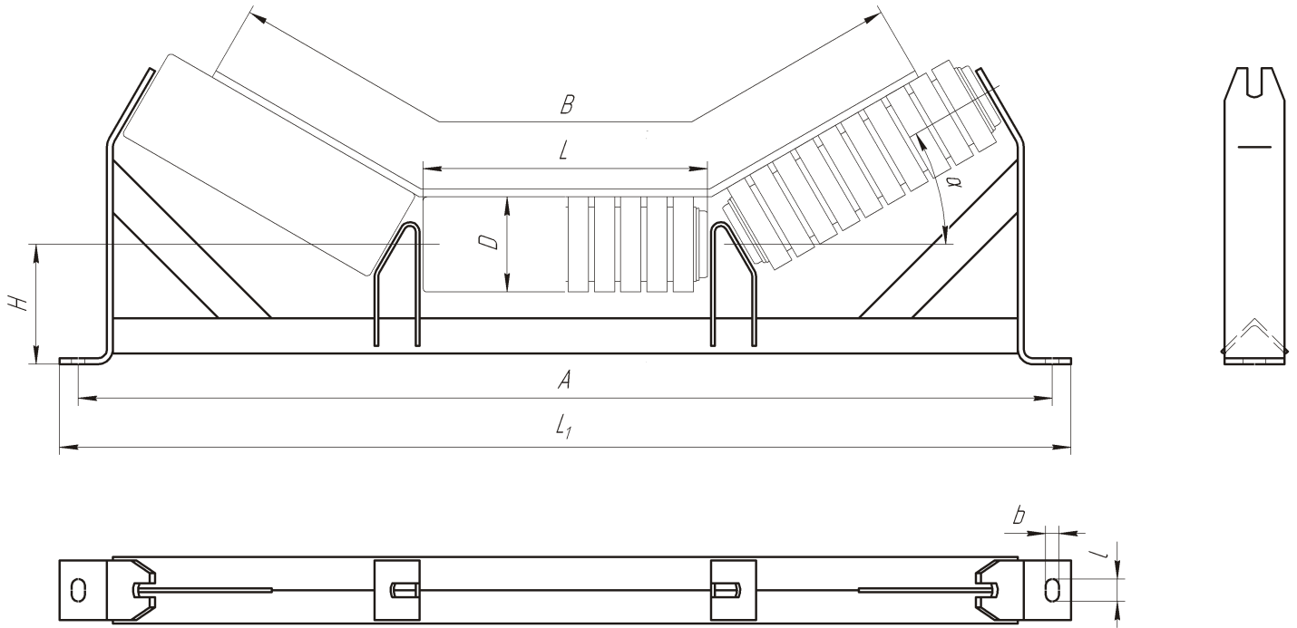
Upper trough roller, type 1
